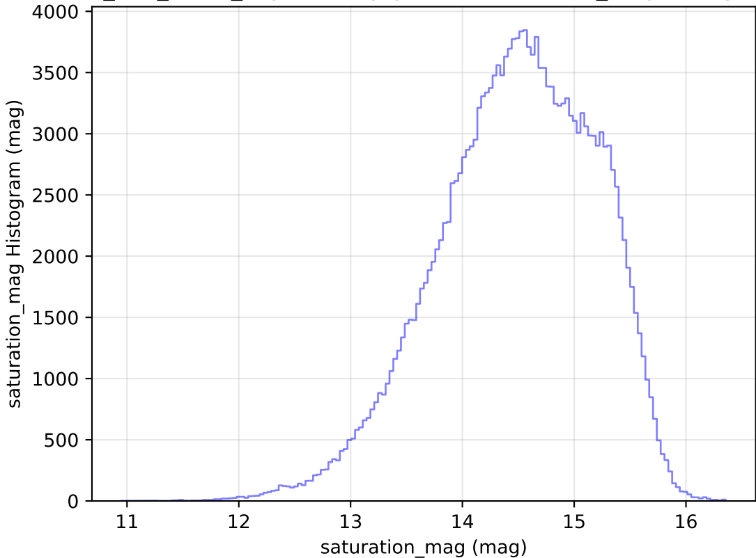
too_100_1v3.4_10yrs All sky g band: saturation_mag Histogram
