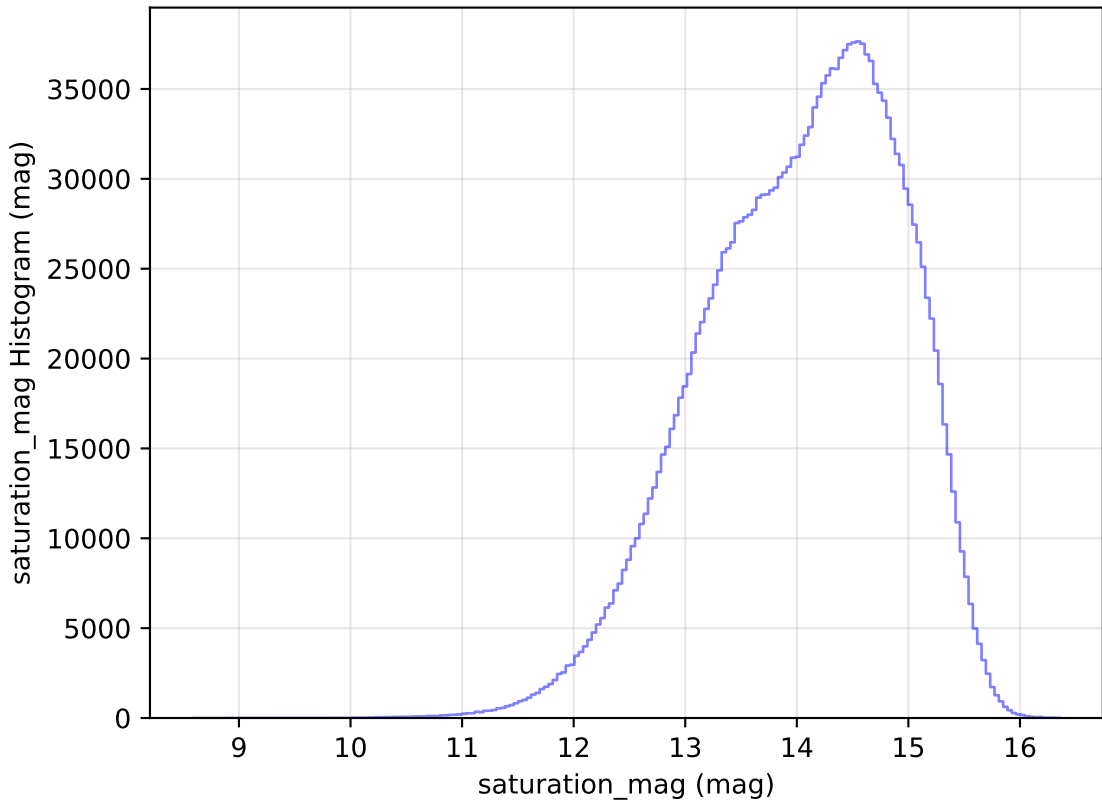
too_100_1v3.4_10yrs All sky all bands: saturation_mag Histogram
