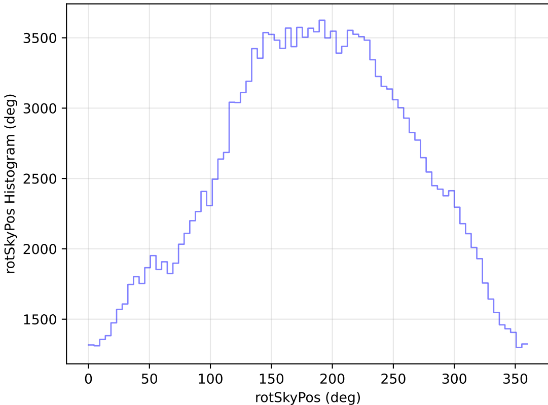
too_100_1v3.4_10yrs WFD g band: rotSkyPos Histogram
