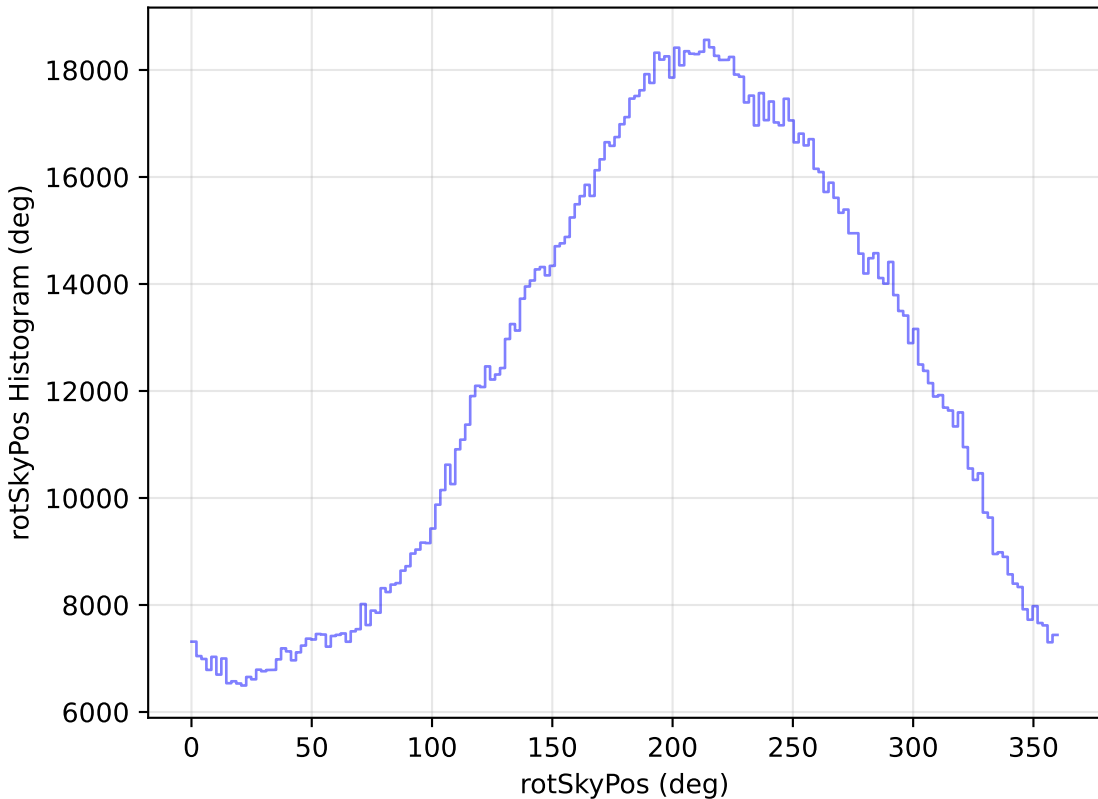
too_100_1v3.4_10yrs WFD all bands: rotSkyPos Histogram
