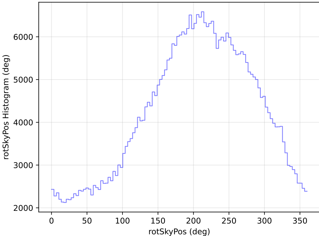
too_100_1v3.4_10yrs All sky z band: rotSkyPos Histogram
