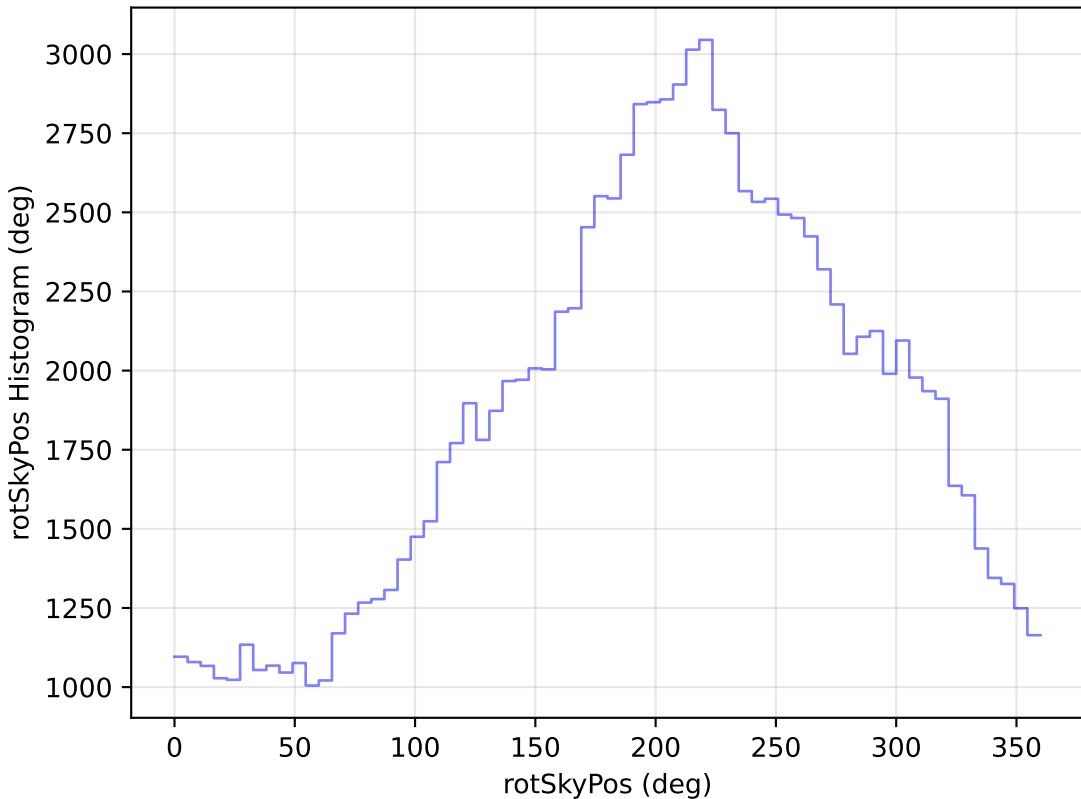
too_100_1v3.4_10yrs All sky u band: rotSkyPos Histogram
