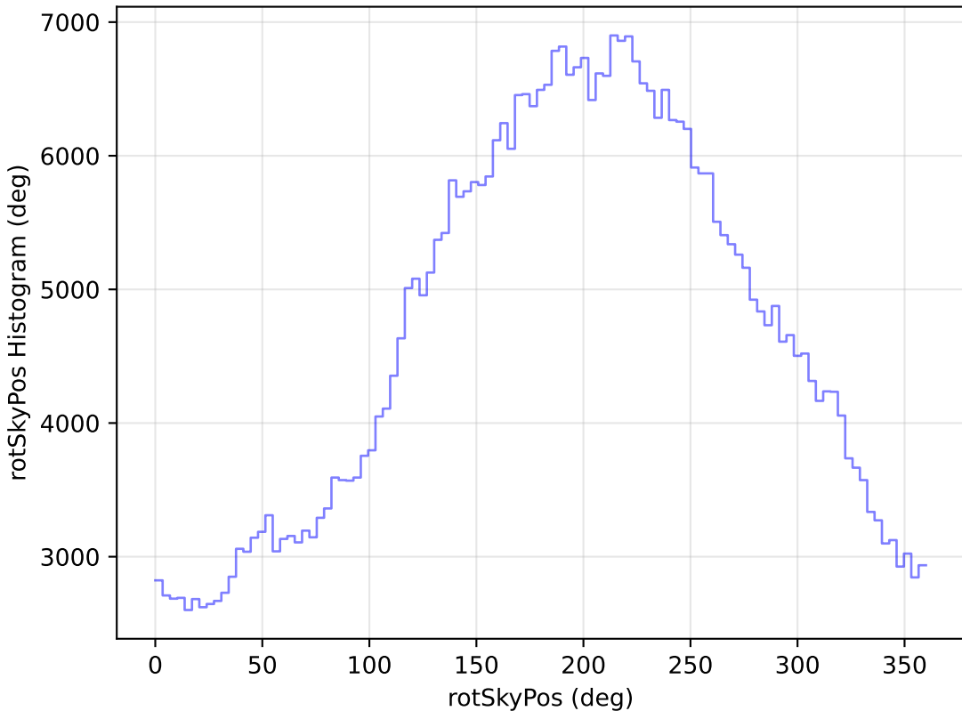
too_100_1v3.4_10yrs All sky r band: rotSkyPos Histogram
