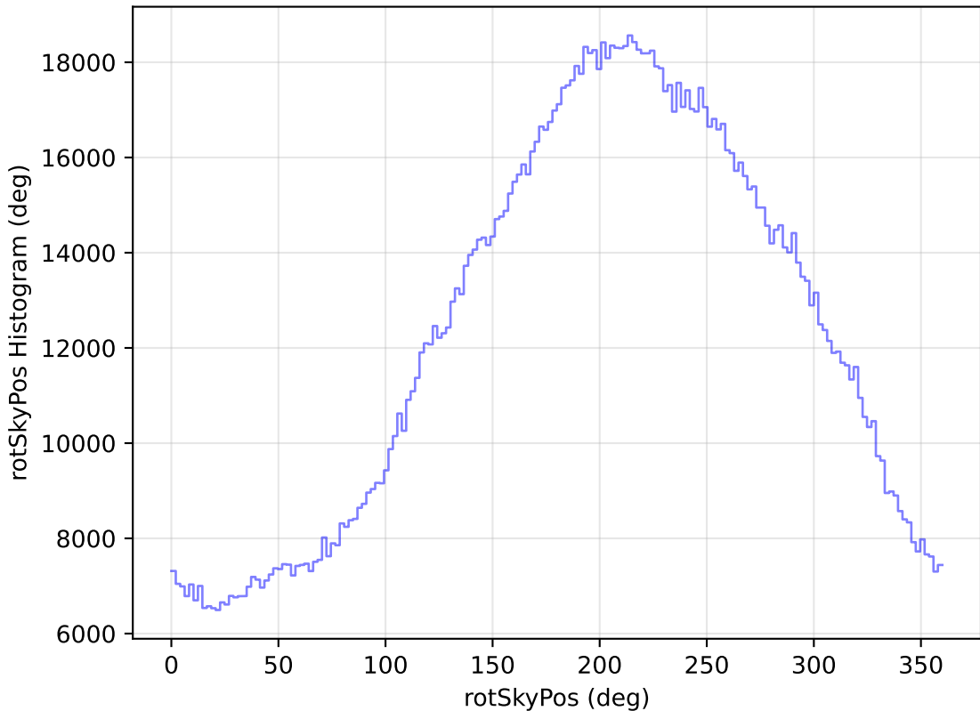
too_100_1v3.4_10yrs All sky all bands: rotSkyPos Histogram
