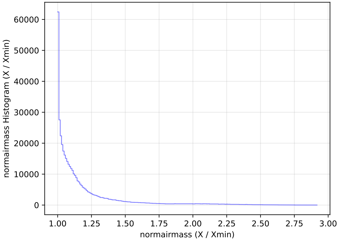
too_100_1v3.4_10yrs WFD z band: normairmass Histogram
