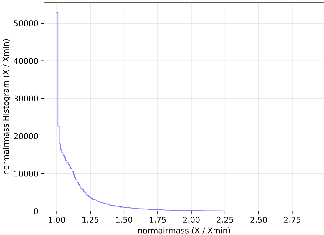
too_100_1v3.4_10yrs WFD y band: normairmass Histogram
