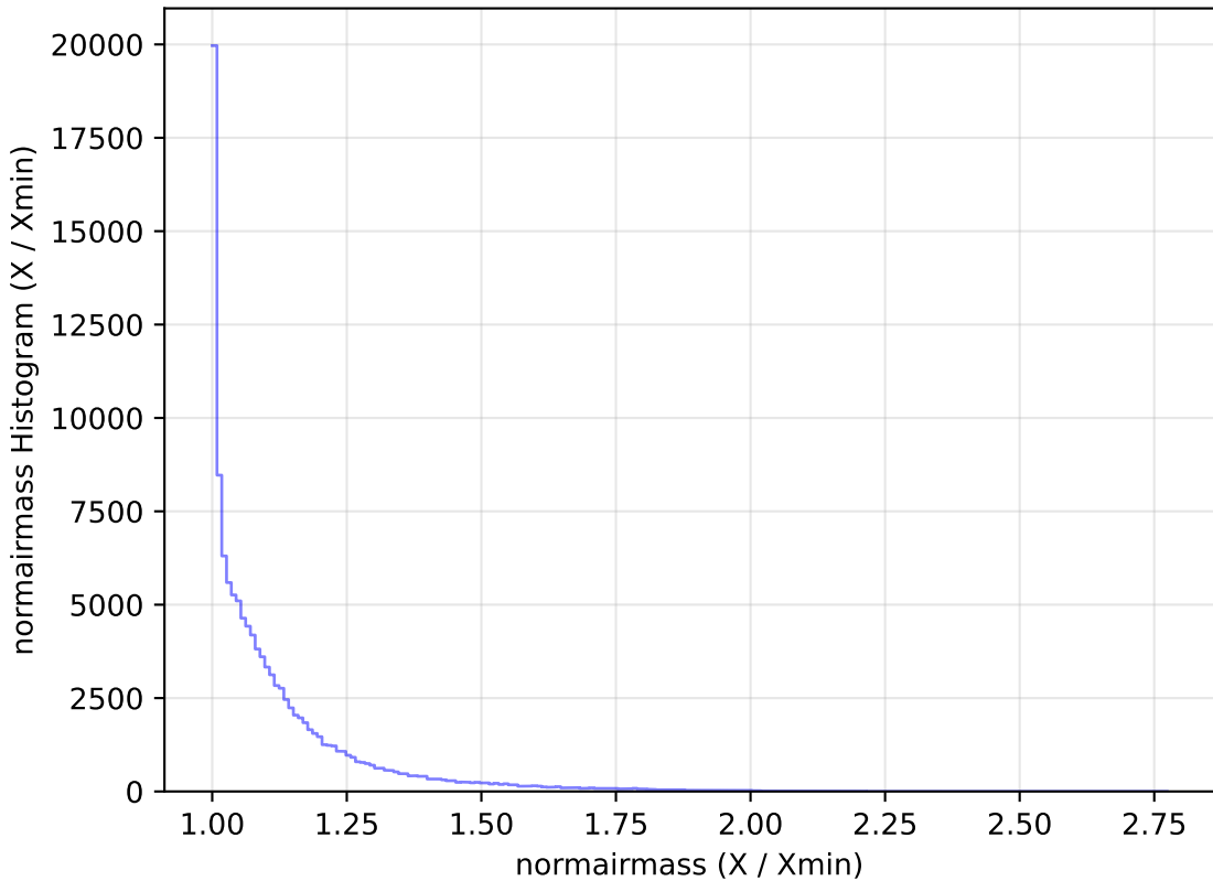
too_100_1v3.4_10yrs WFD u band: normairmass Histogram
