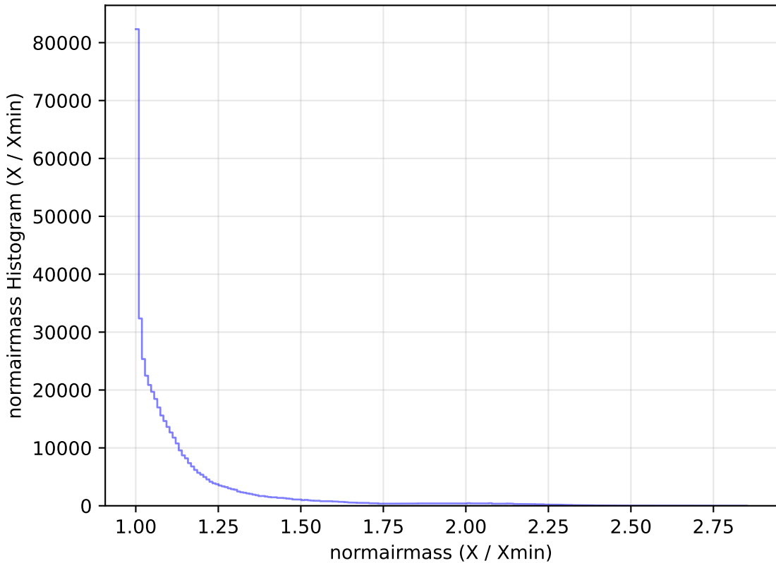
too_100_1v3.4_10yrs WFD r band: normairmass Histogram
