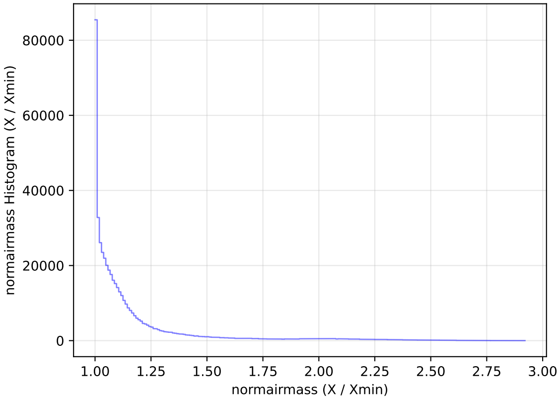
too_100_1v3.4_10yrs WFD i band: normairmass Histogram
