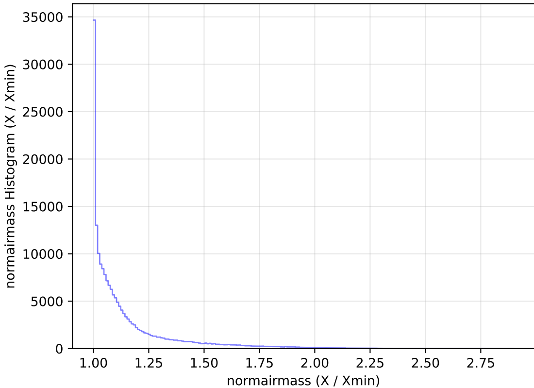
too_100_1v3.4_10yrs WFD g band: normairmass Histogram
