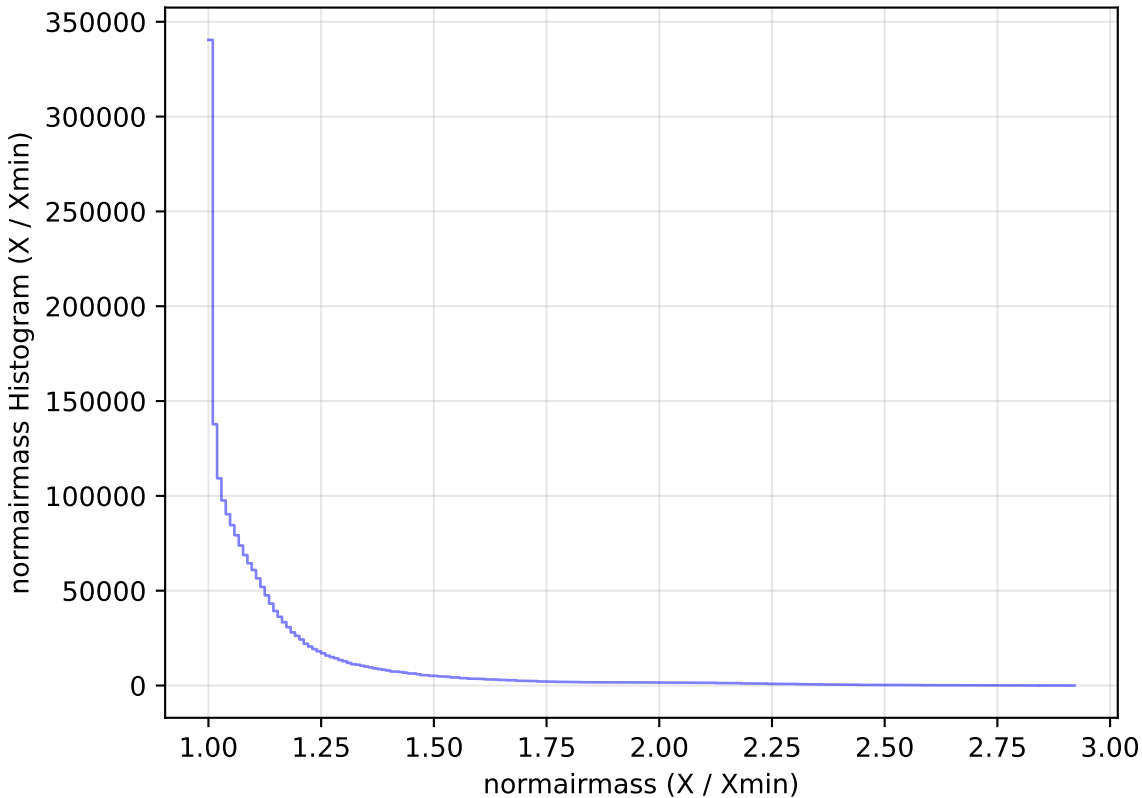
too_100_1v3.4_10yrs WFD all bands: normairmass Histogram
