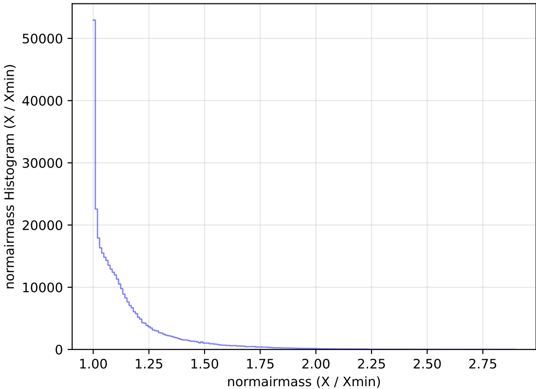
too_100_1v3.4_10yrs All sky y band: normairmass Histogram
