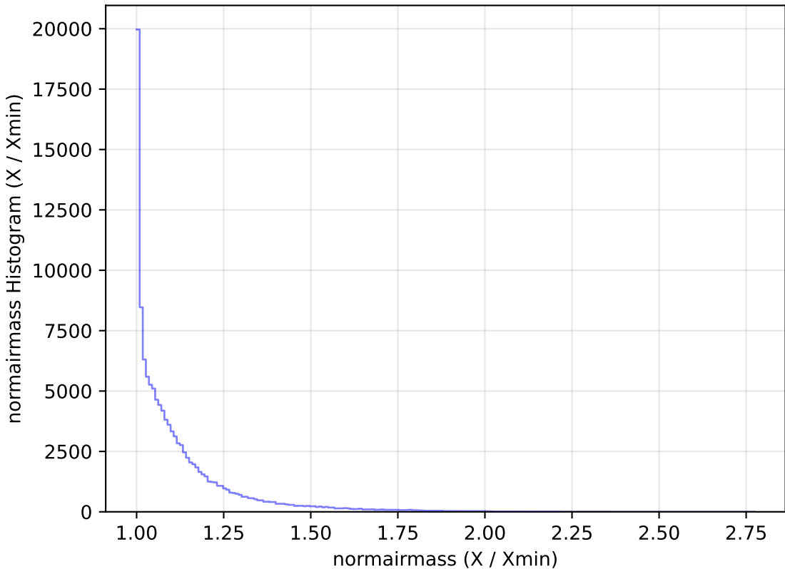
too_100_1v3.4_10yrs All sky u band: normairmass Histogram
