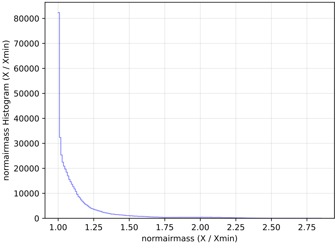
too_100_1v3.4_10yrs All sky r band: normairmass Histogram
