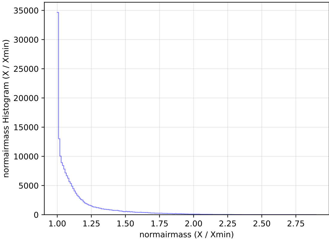
too_100_1v3.4_10yrs All sky g band: normairmass Histogram
