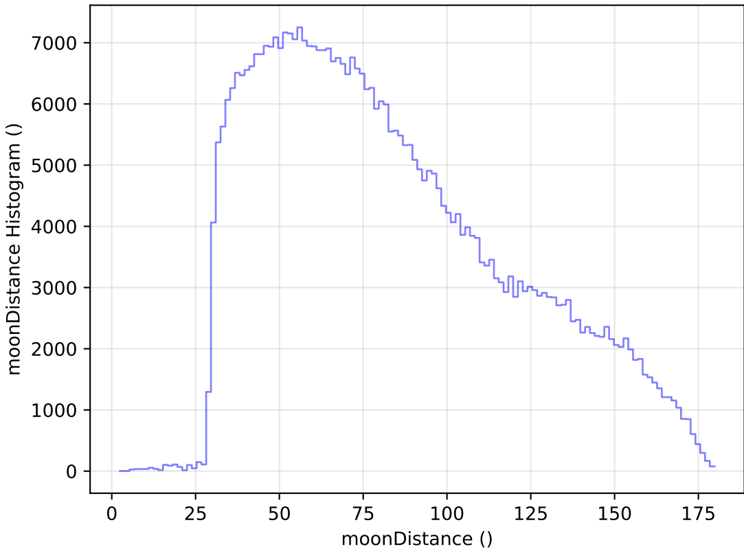
too_100_1v3.4_10yrs WFD z band: moonDistance Histogram
