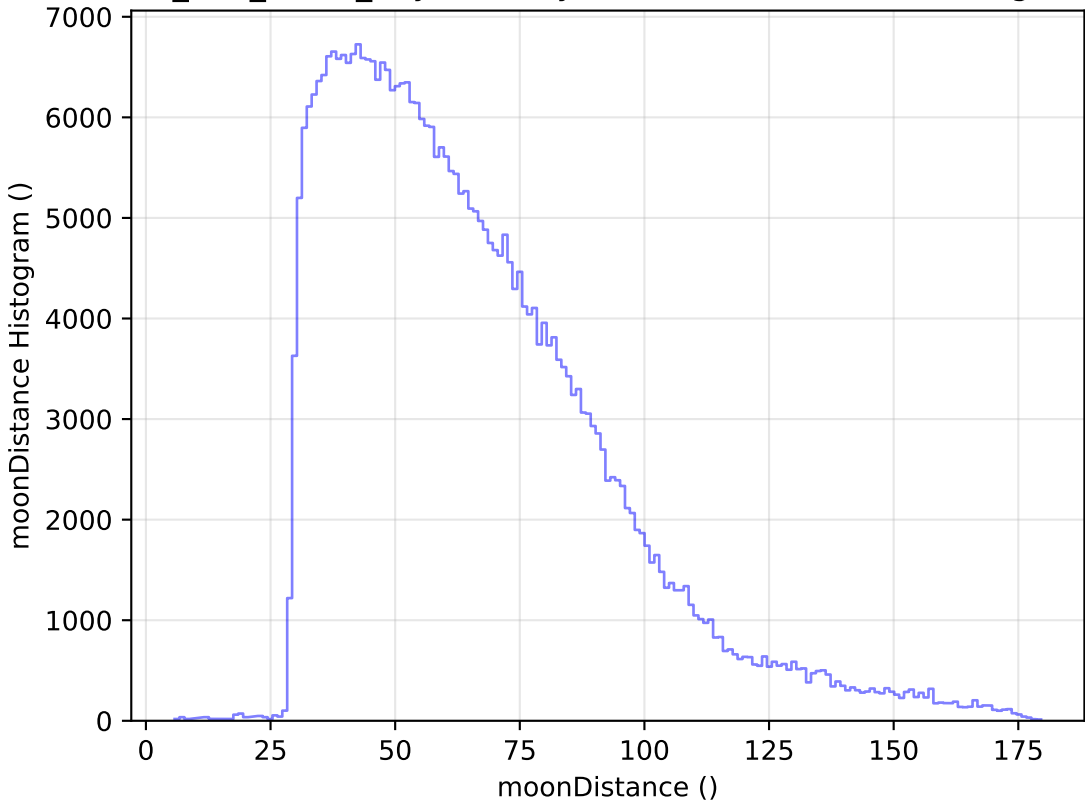
too_100_1v3.4_10yrs WFD y band: moonDistance Histogram
