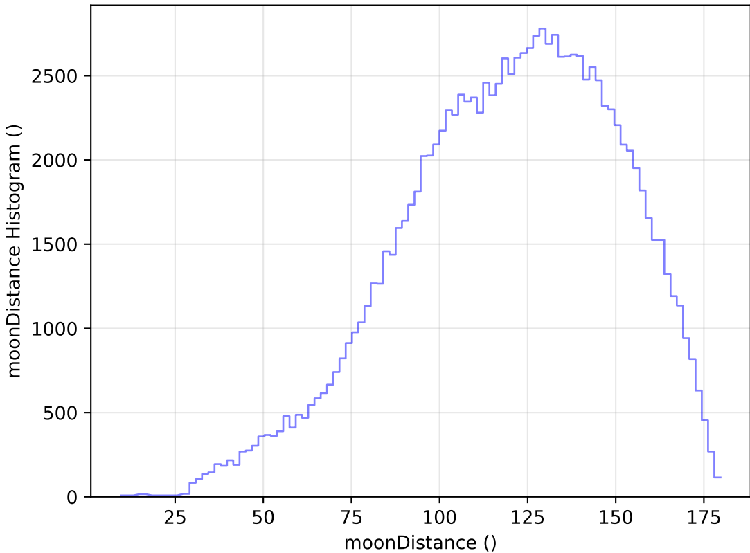
too_100_1v3.4_10yrs WFD u band: moonDistance Histogram
