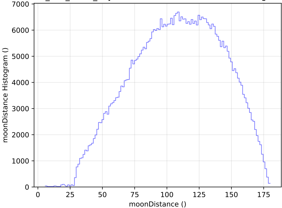
too_100_1v3.4_10yrs WFD r band: moonDistance Histogram
