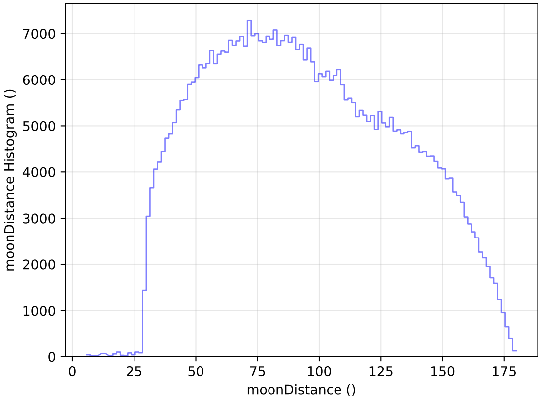
too_100_1v3.4_10yrs WFD i band: moonDistance Histogram
