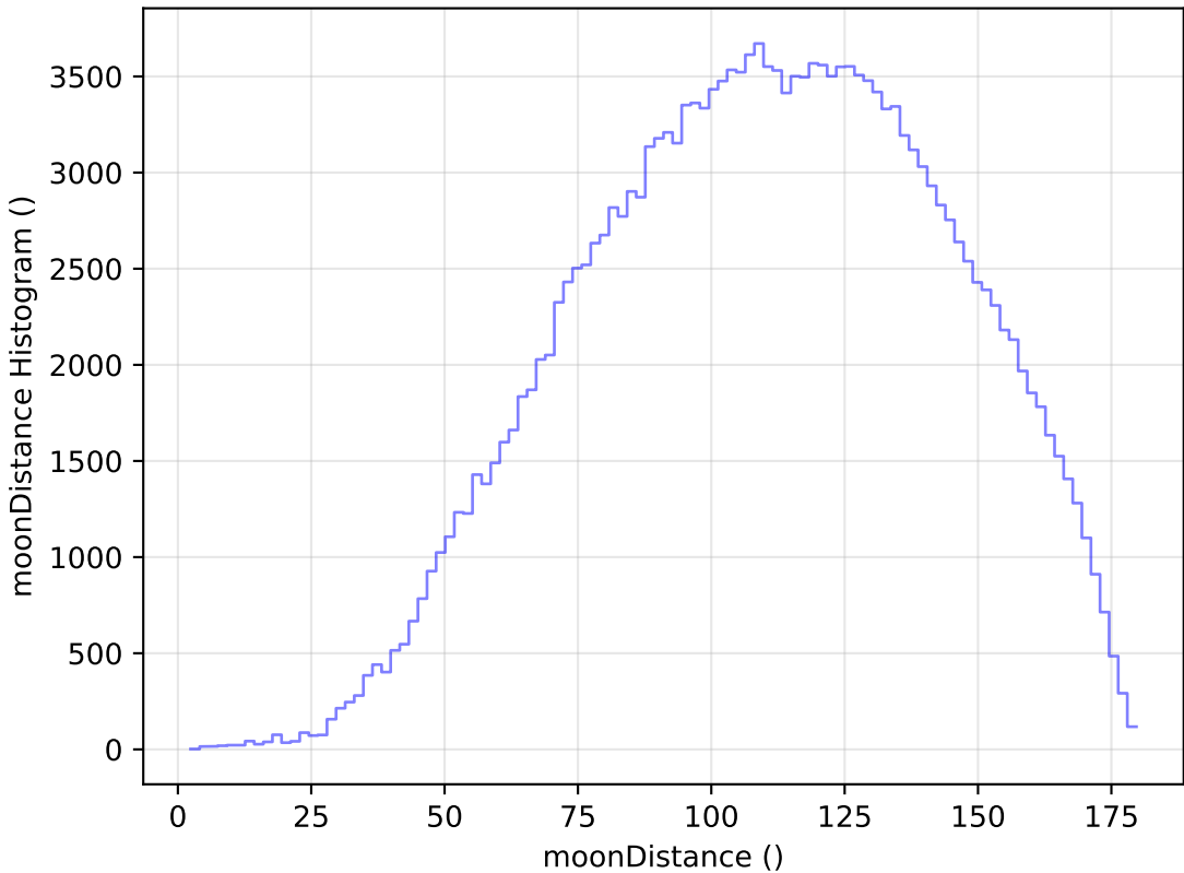
too_100_1v3.4_10yrs WFD g band: moonDistance Histogram
