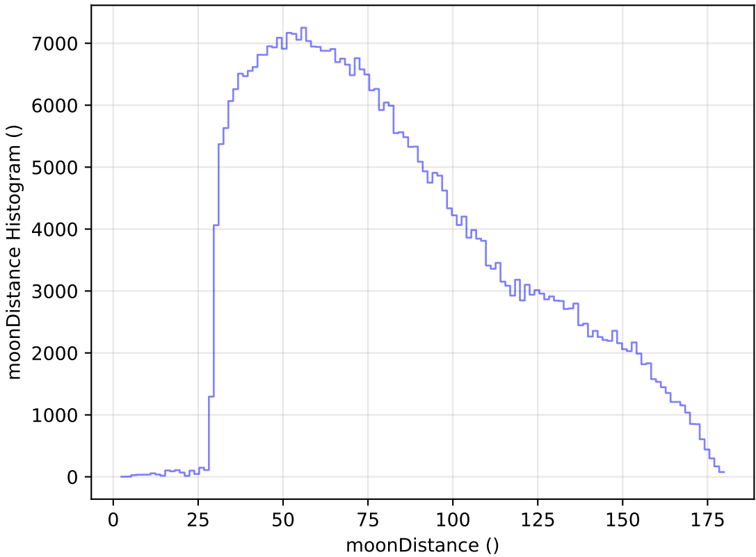
too_100_1v3.4_10yrs All sky z band: moonDistance Histogram
