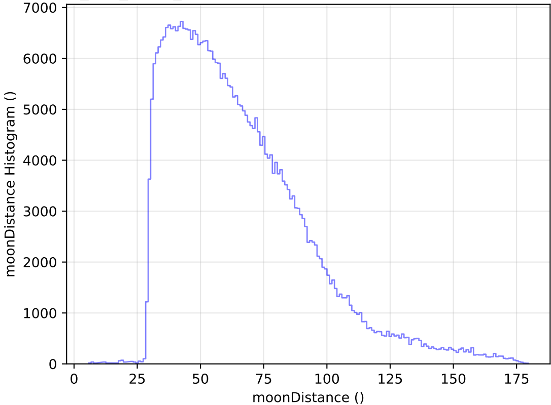
too_100_1v3.4_10yrs All sky y band: moonDistance Histogram
