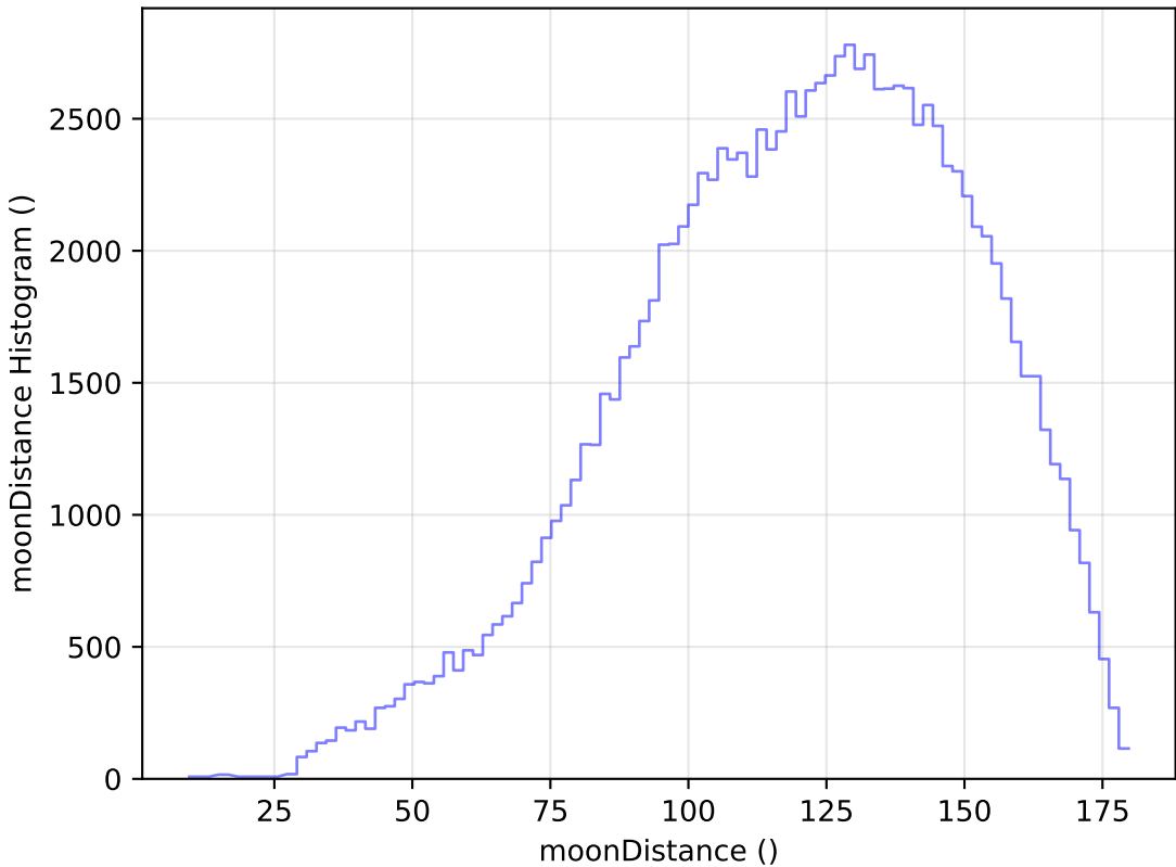
too_100_1v3.4_10yrs All sky u band: moonDistance Histogram
