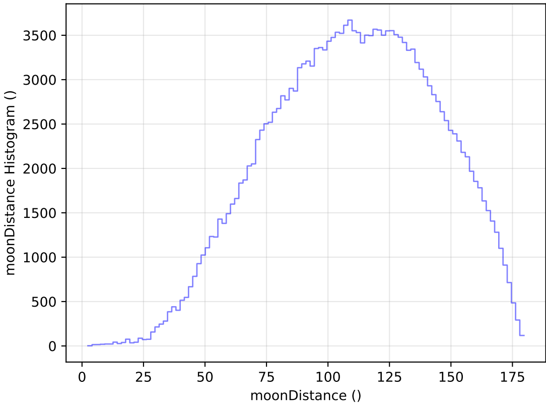
too_100_1v3.4_10yrs All sky g band: moonDistance Histogram
