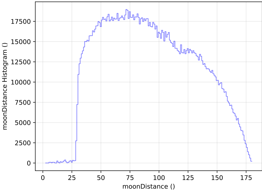
too_100_1v3.4_10yrs All sky all bands: moonDistance Histogram
