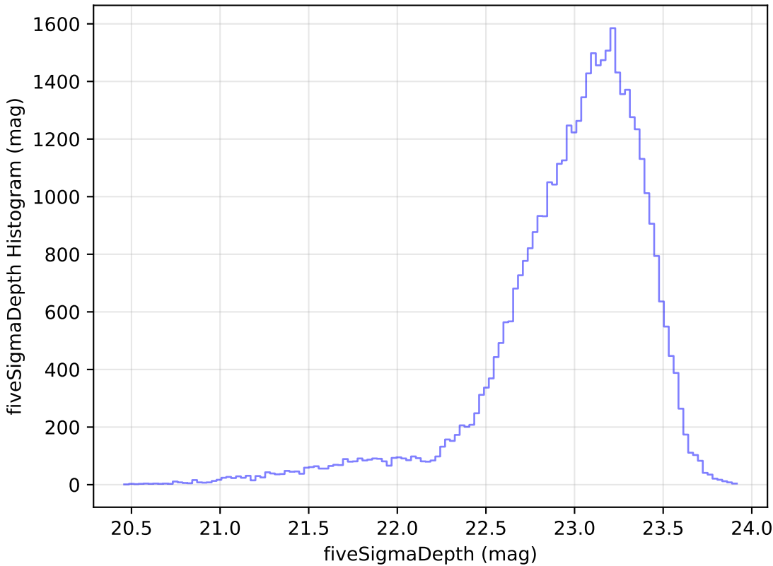
too_100_1v3.4_10yrs Yr 1 z band: fiveSigmaDepth Histogram
