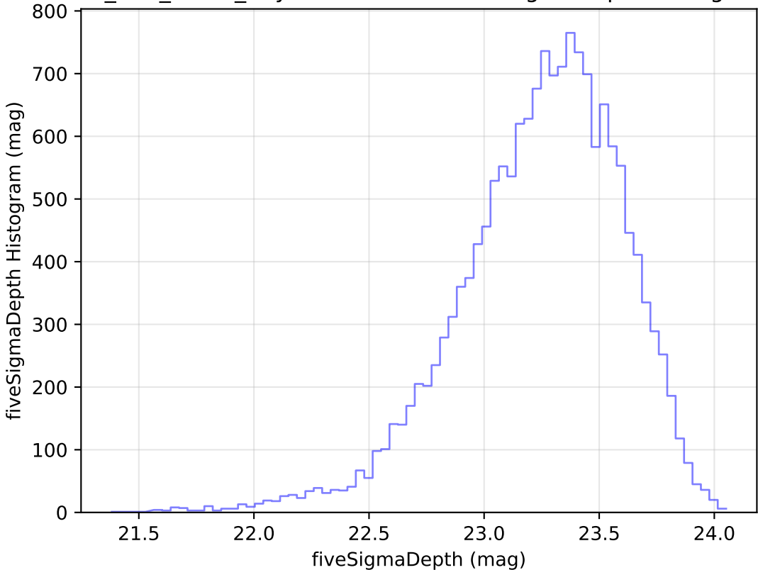
too_100_1v3.4_10yrs Yr 1 u band: fiveSigmaDepth Histogram
