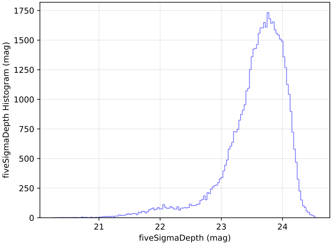
too_100_1v3.4_10yrs Yr 1 i band: fiveSigmaDepth Histogram
