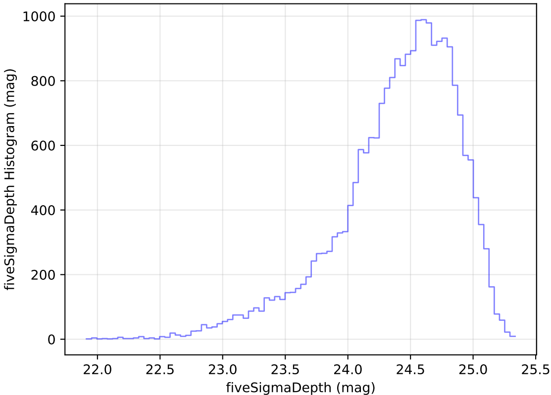
too_100_1v3.4_10yrs Yr 1 g band: fiveSigmaDepth Histogram
