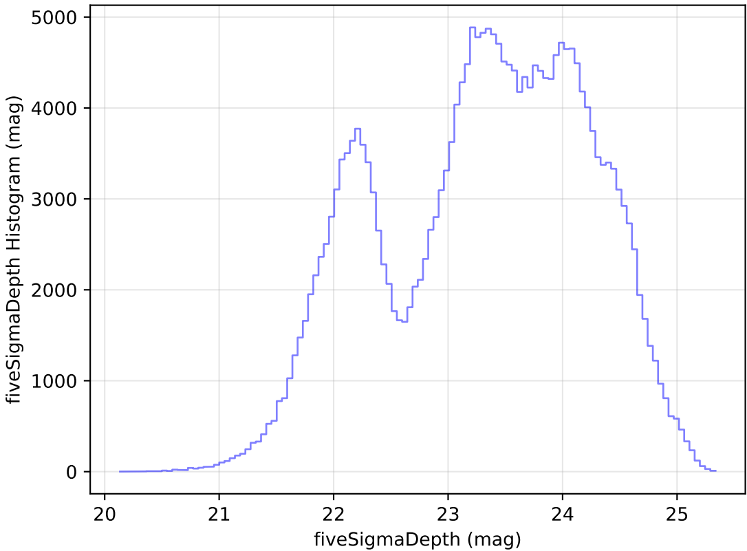
too_100_1v3.4_10yrs Yr 1 all bands: fiveSigmaDepth Histogram
