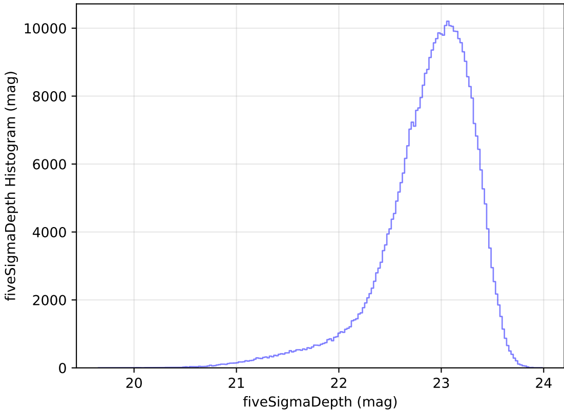
too_100_1v3.4_10yrs WFD z band: fiveSigmaDepth Histogram
