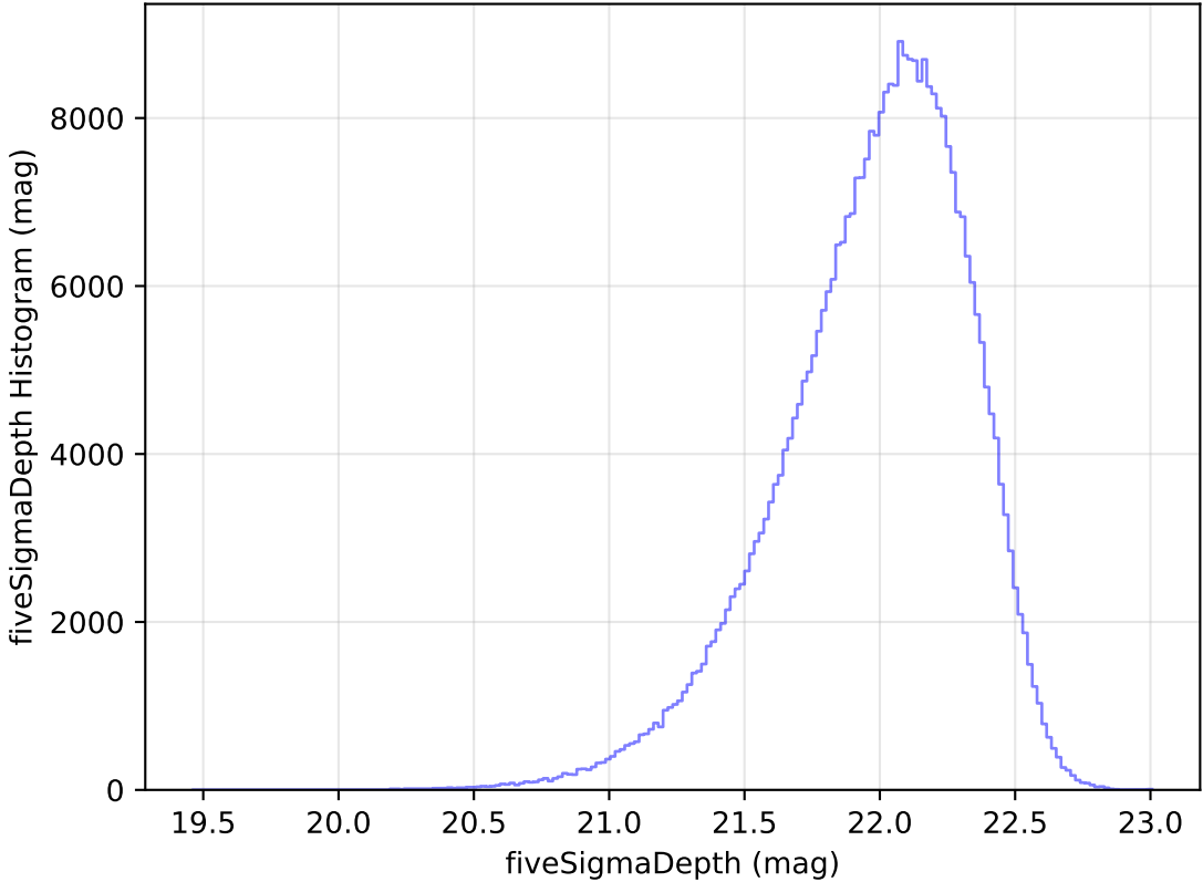
too_100_1v3.4_10yrs WFD y band: fiveSigmaDepth Histogram
