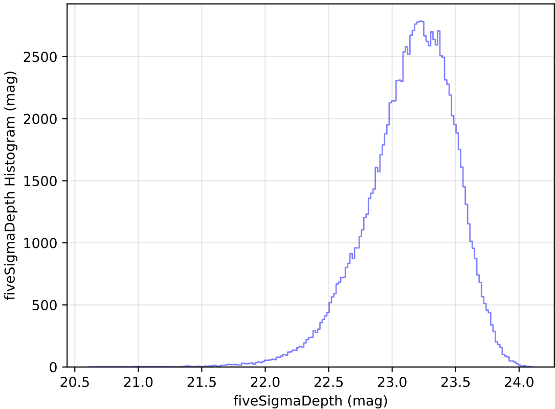
too_100_1v3.4_10yrs WFD u band: fiveSigmaDepth Histogram
