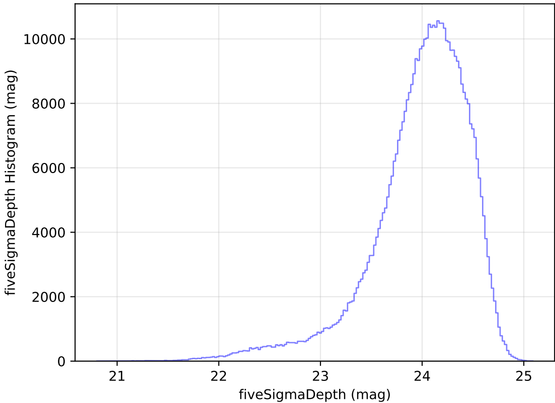
too_100_1v3.4_10yrs WFD r band: fiveSigmaDepth Histogram
