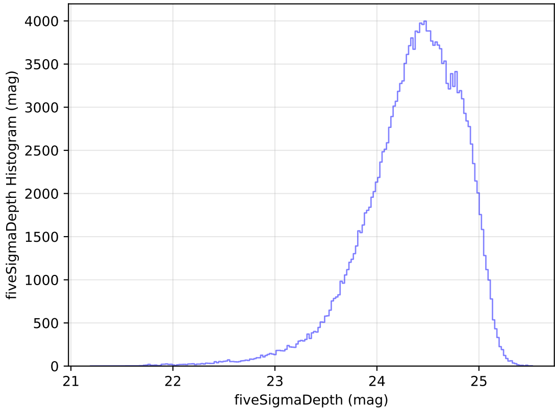
too_100_1v3.4_10yrs WFD g band: fiveSigmaDepth Histogram
