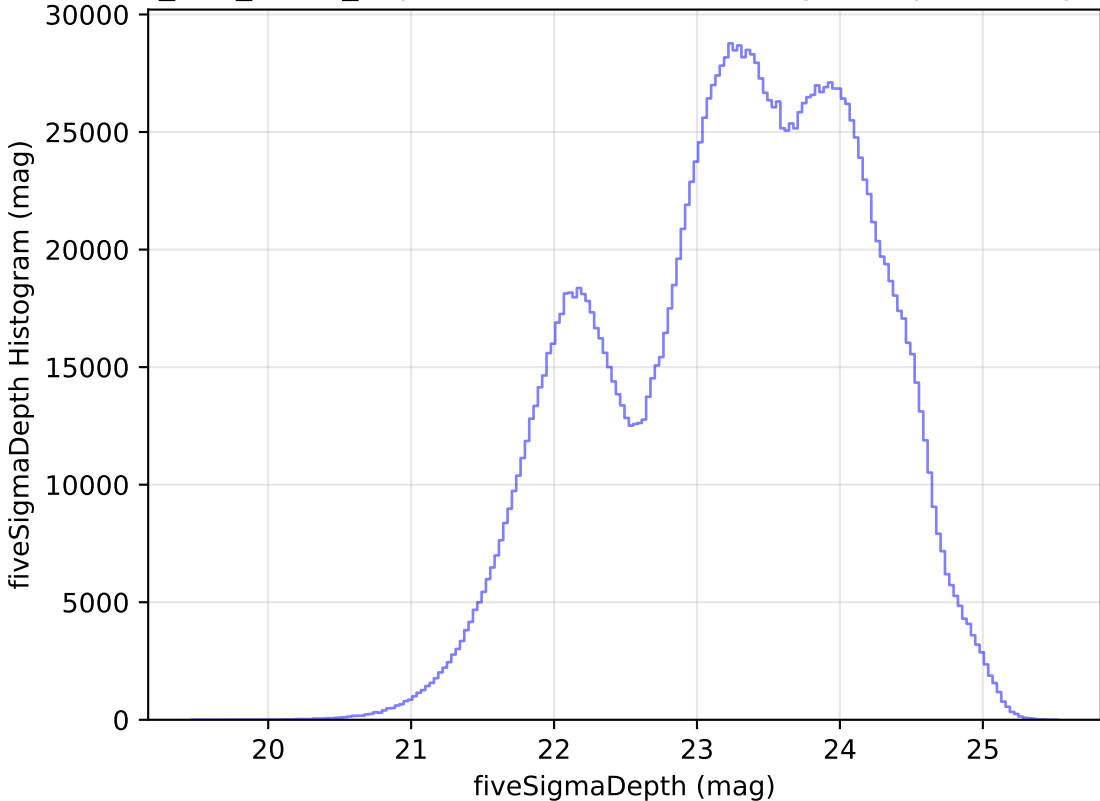
too_100_1v3.4_10yrs WFD all bands: fiveSigmaDepth Histogram
