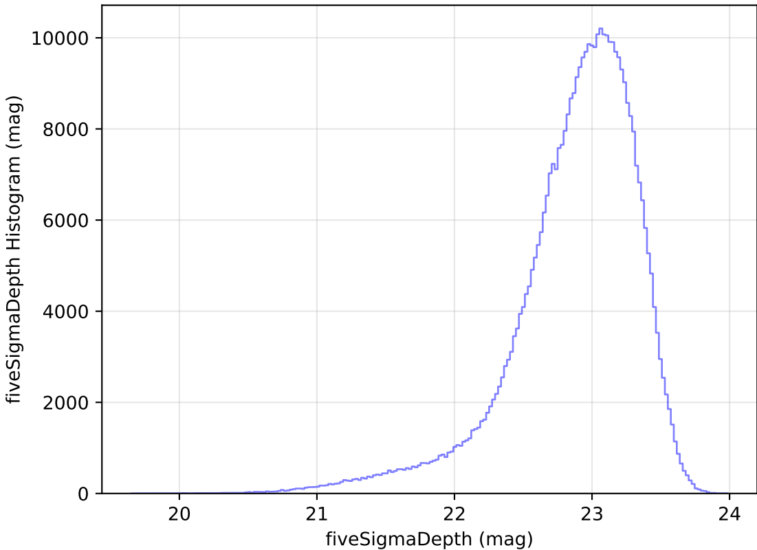
too_100_1v3.4_10yrs All sky z band: fiveSigmaDepth Histogram
