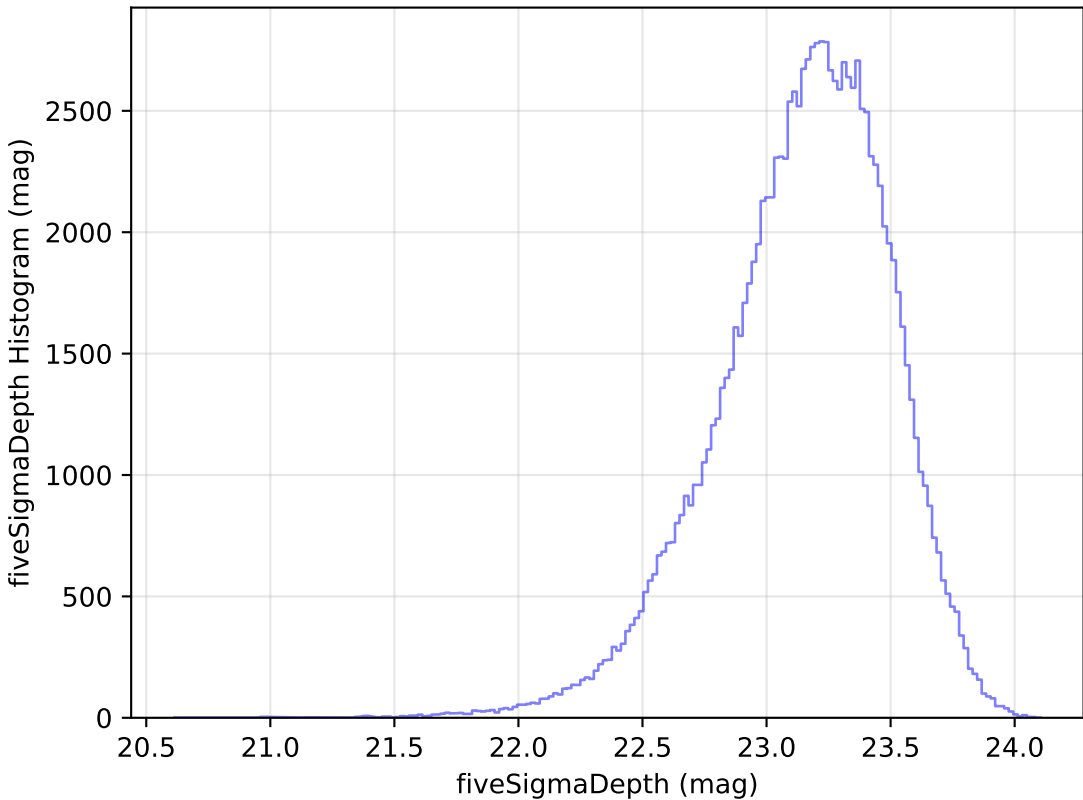
too_100_1v3.4_10yrs All sky u band: fiveSigmaDepth Histogram
