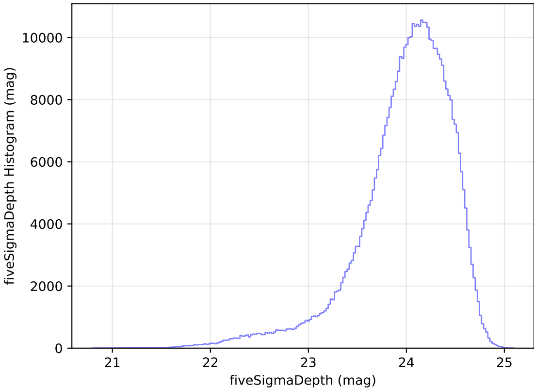
too_100_1v3.4_10yrs All sky r band: fiveSigmaDepth Histogram
