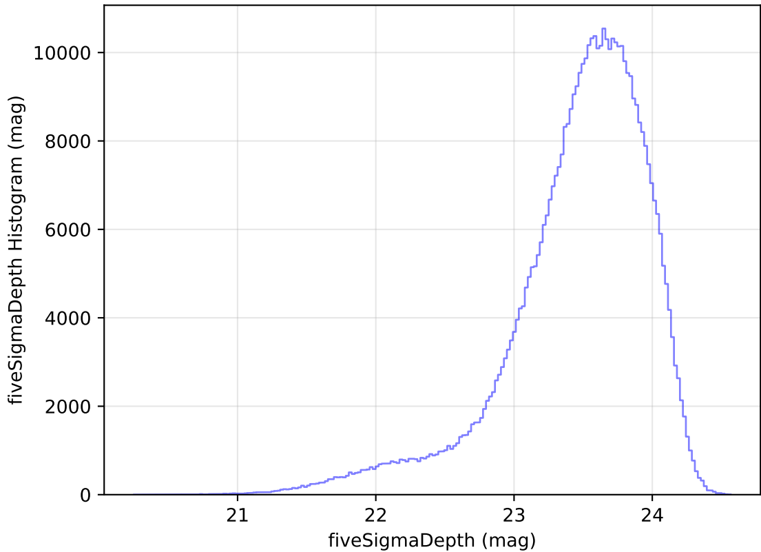
too_100_1v3.4_10yrs All sky i band: fiveSigmaDepth Histogram
