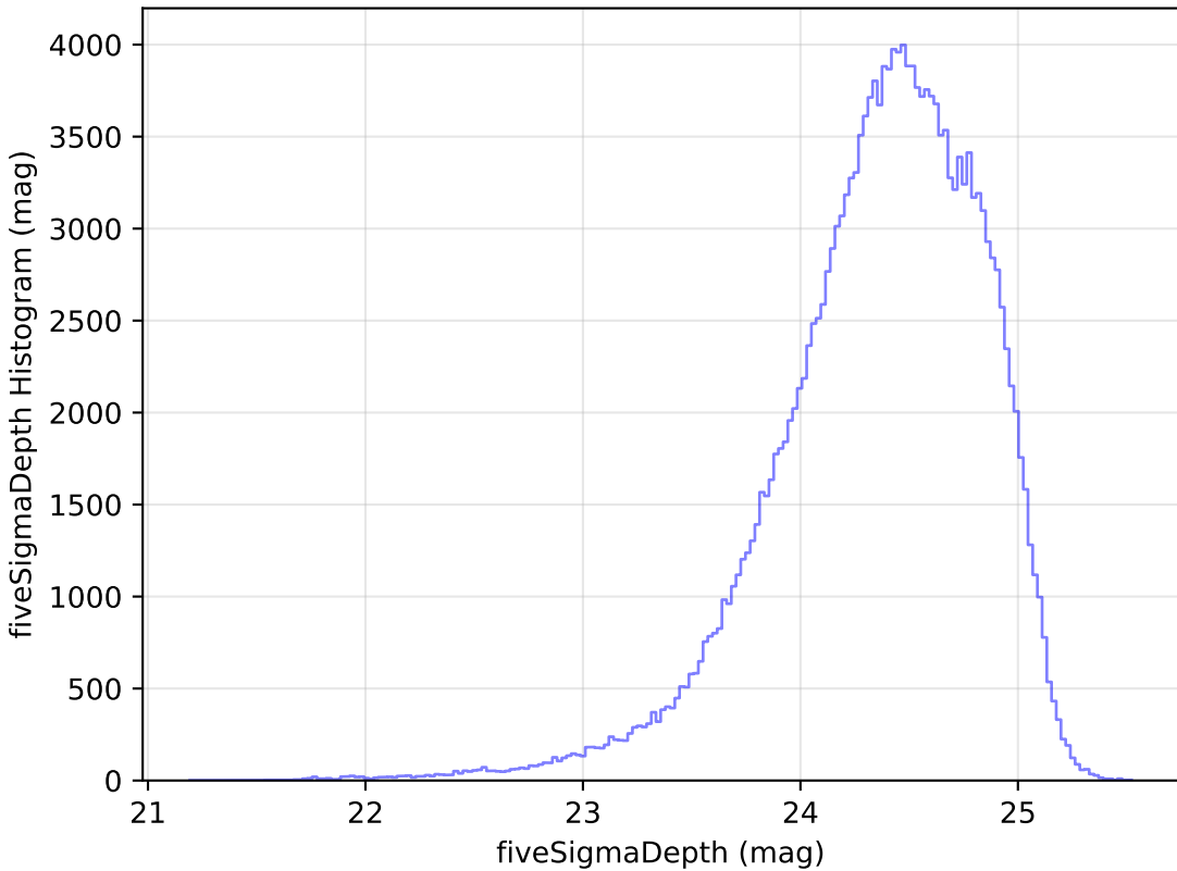
too_100_1v3.4_10yrs All sky g band: fiveSigmaDepth Histogram
