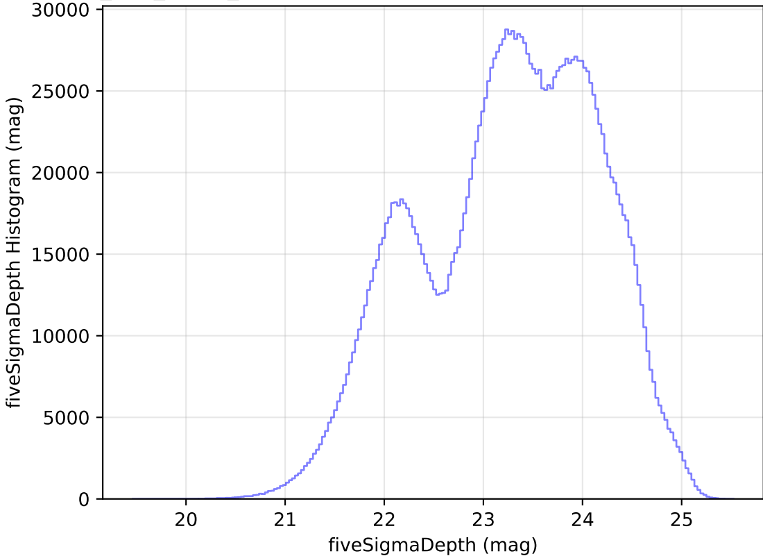
too_100_1v3.4_10yrs All sky all bands: fiveSigmaDepth Histogram
