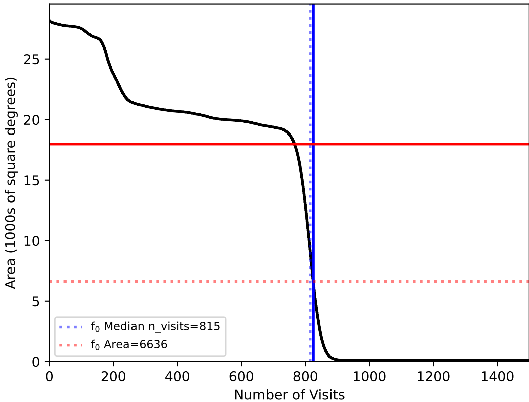
too_100_1v3.4_10yrs All sky: fO
