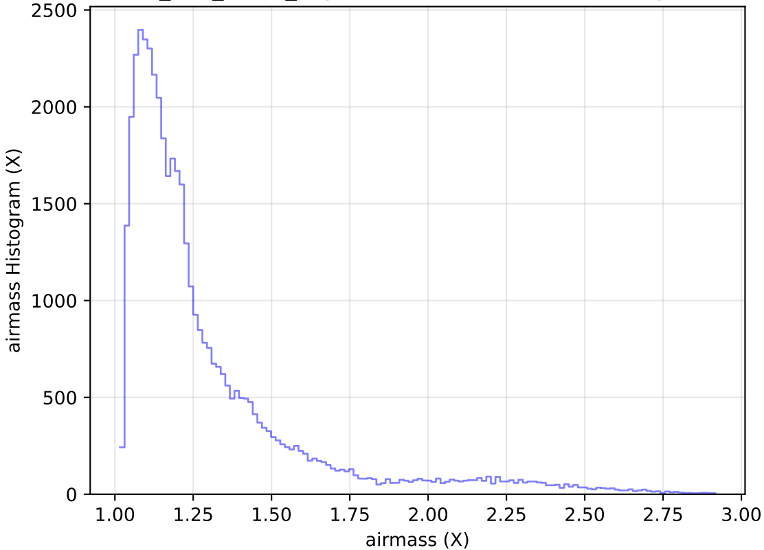
too_100_1v3.4_10yrs Yr 1 z band: airmass Histogram
