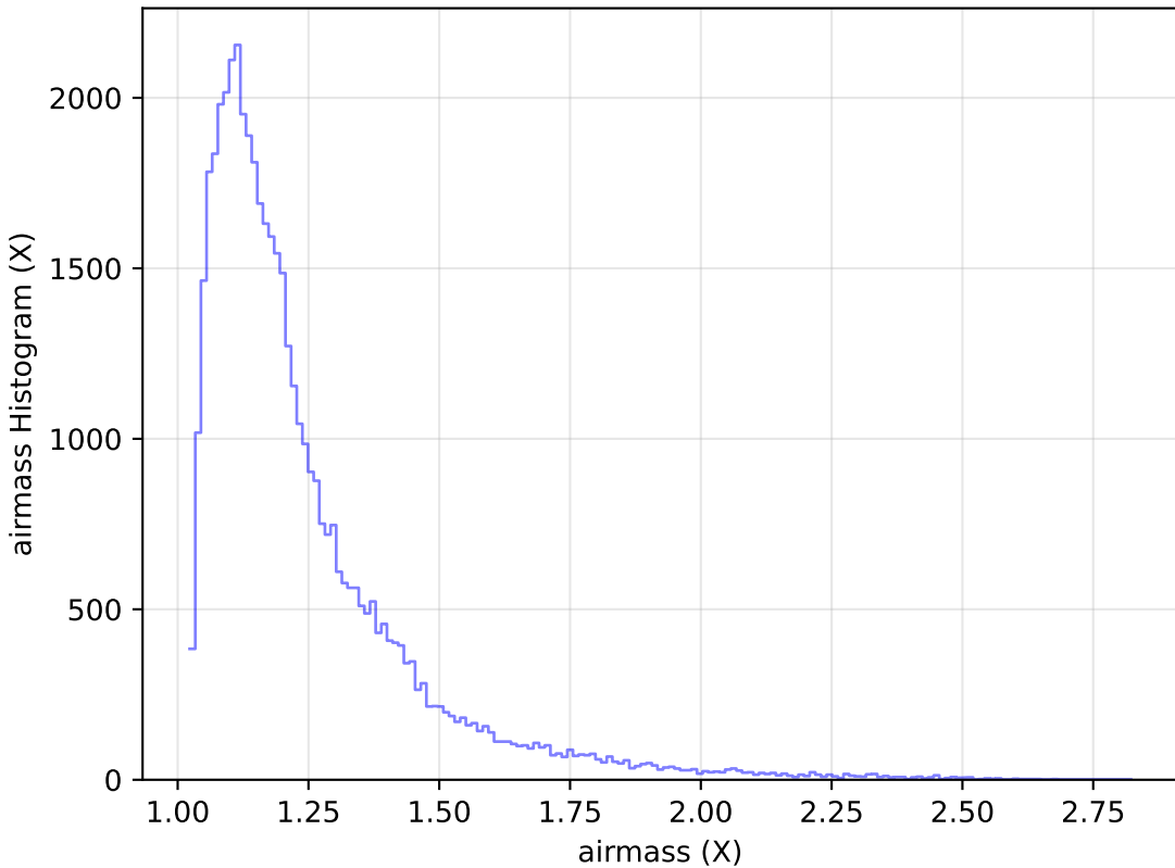
too_100_1v3.4_10yrs Yr 1 y band: airmass Histogram
